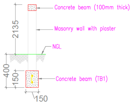
wall detail
